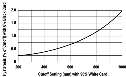
Figure 11. Hysteresis
