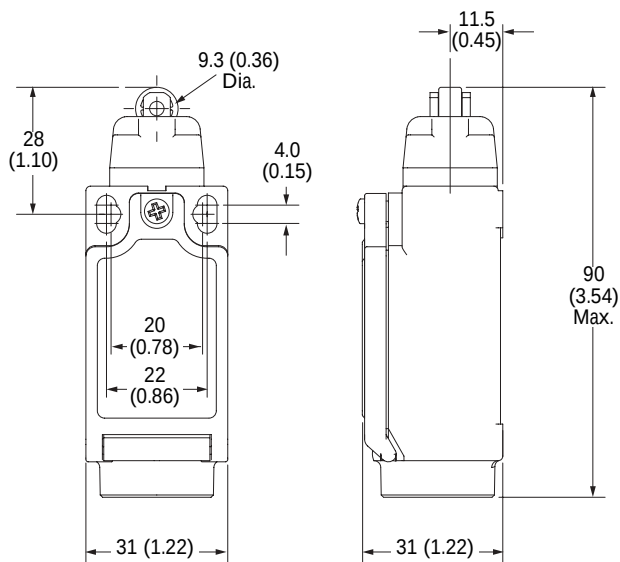
Roller Plunger
