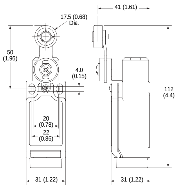
Short Lever
