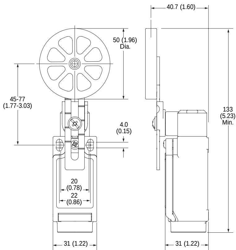
Rubber Roller
