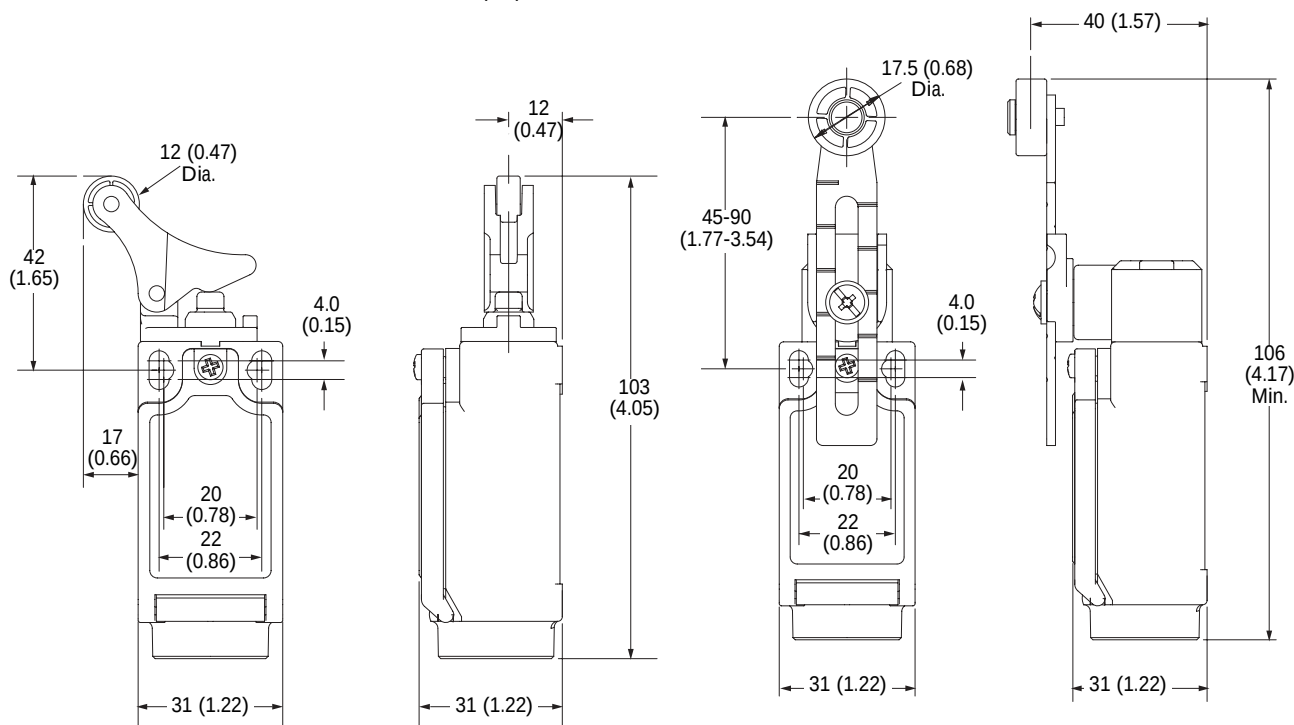
Offset Hinge
