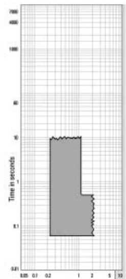
Digitrip 520Mi/520Mi Long and short delay curve
