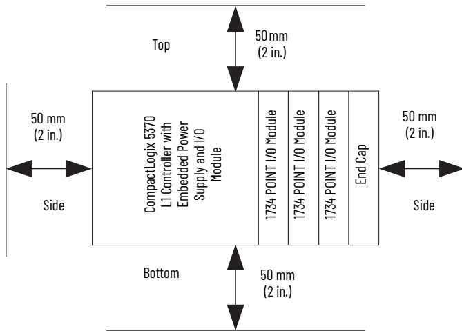
CompactLogix 5370 L1 Controllers
