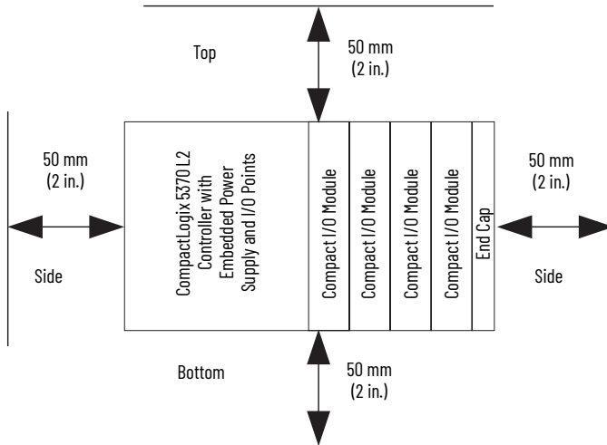
CompactLogix 5370 L2 Controllers
