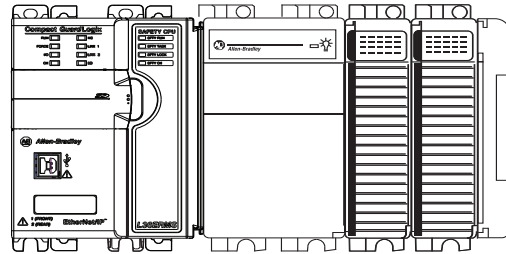
Compact GuardLogix 5370 Control System
